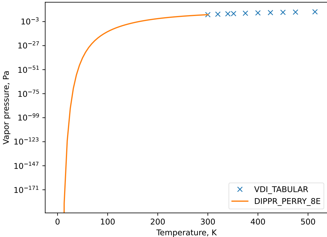
Vapor pressure of 64-17-5
