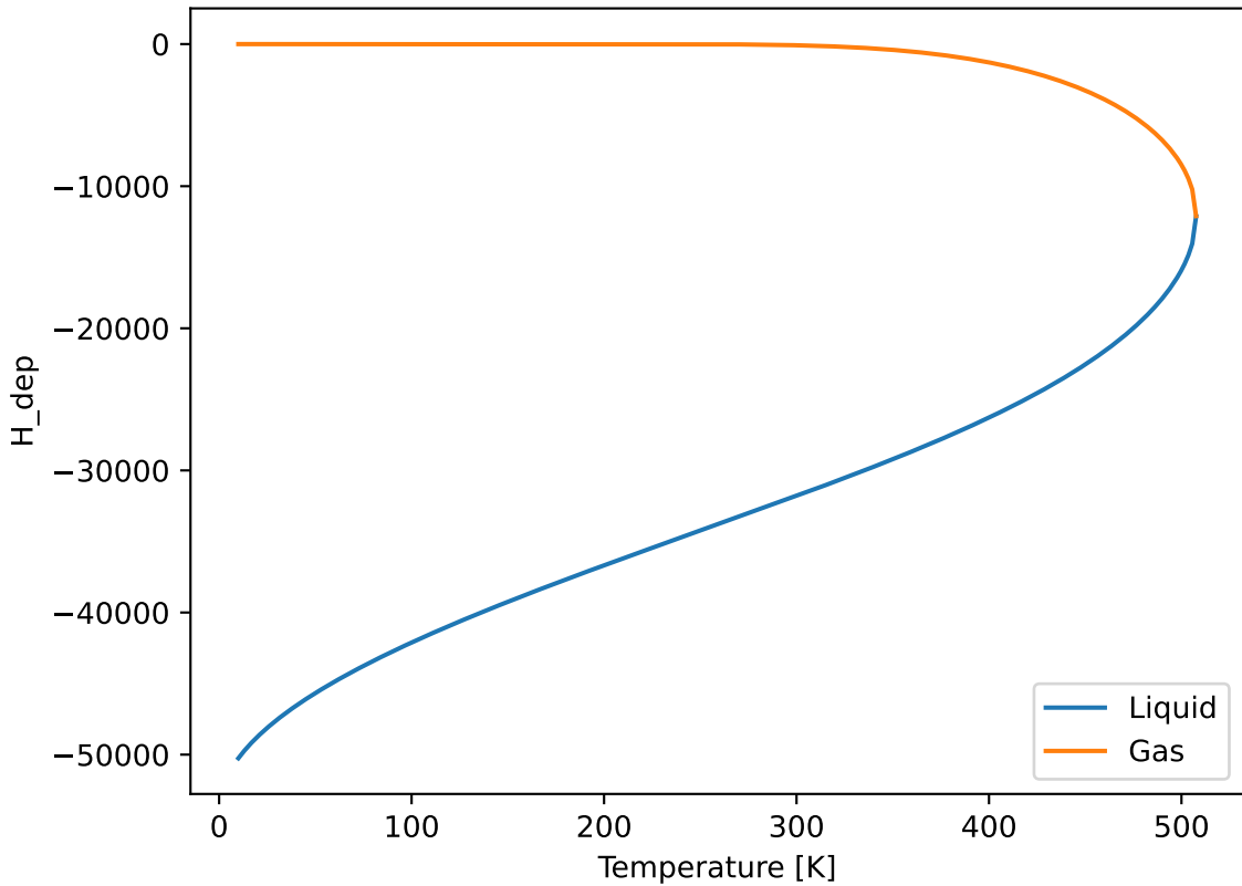
Saturation H_dep curve
